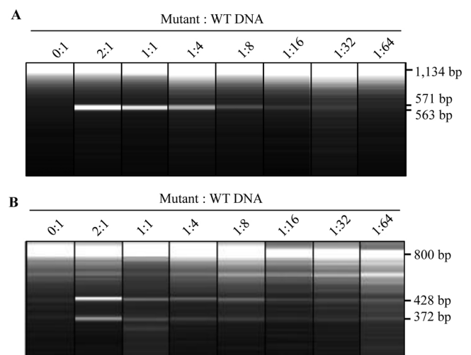
Fig. 4. The sensitivity of GFP-CELI-His in combination with the MD buffer in detecting mismatches. Genomic DNAs isolated from two different rice mutants with mutations in Os04g0650600 (A) and Os03g0167600 (B) were mixed with the DNA from the wildtype in different ratios (0:1, 2:1, 1:1, 1:4, 1:8, 1:16, 1:32, 1:64), used for PCR amplifications and mismatch detection using GFP-CELI-His in optimized MD buffer. Note that the mutation could be detected with a high sensitivity in 1:32 mixed templates. Sizes of DNA fragments are indicated at the side.
